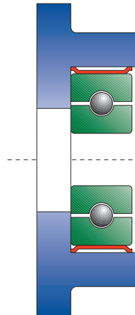
Outer bearing mount in tub base housing
