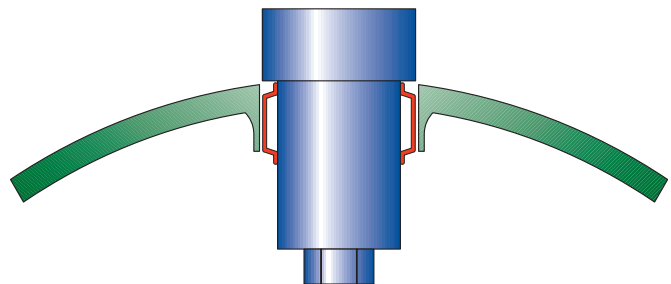
Inner race bearing mount on alloy shaft
