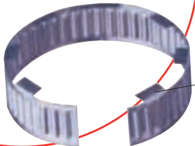
Tabs on the ANT22X7S1 prevent the tolerance ring from moving axially
