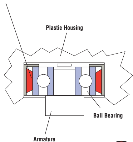
Tabs on the ANT22X7S1 prevent the tolerance ring from moving axially
